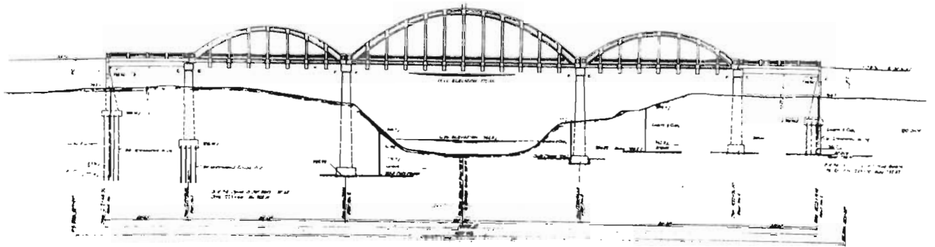
Pottawatomie Creek Bridge from original plans.
